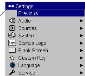
Settings menu
